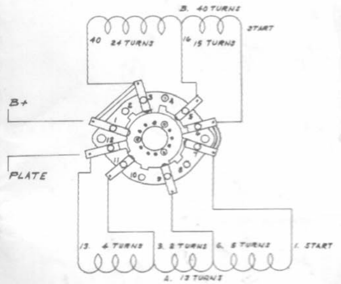
REAR VIEW OF 2A TURRET SWITCH CONNECTIONS
